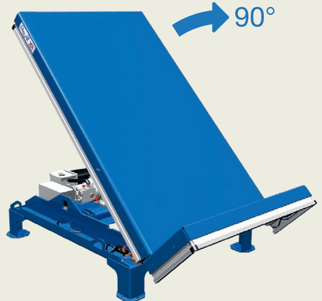
EDLF 65 has double-acting hydraulics and 90° tilting over short side.
