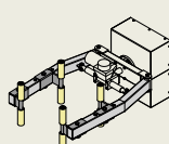
Drum turner 87924 equipped with Gripper A
